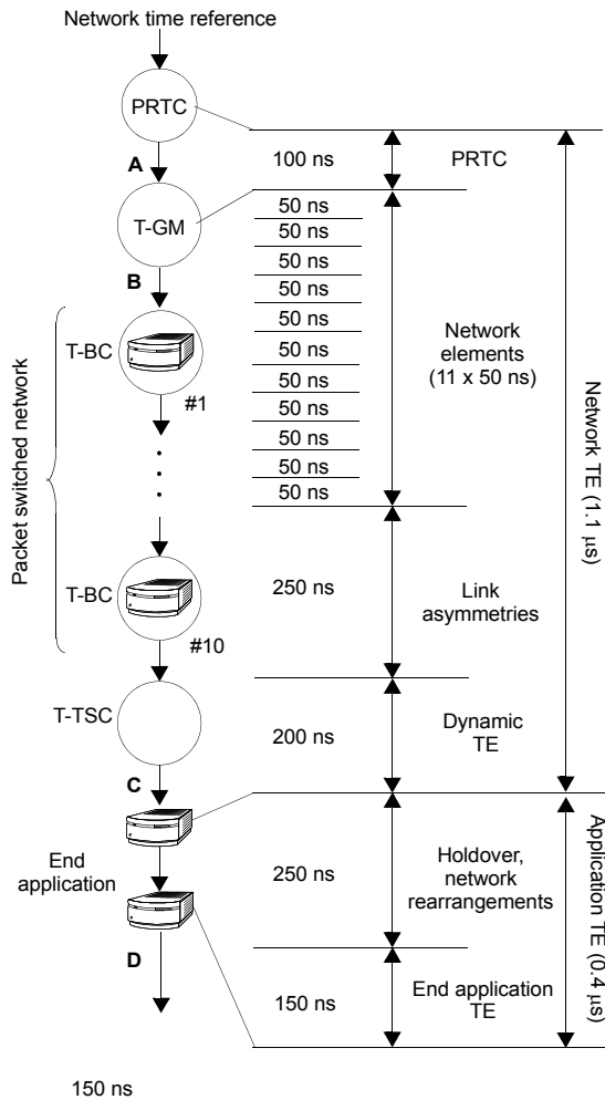
Figure 18 Time Error budget in a phase / time delivery application. TE control requires careful planning in these applications.
