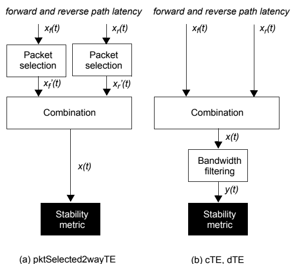
Figure 21 ITU-T G.8260 metrics derived from the raw TE: (a) pktSelected2wayTE , (b) cTE and dTE. The bandwidth filter is a 0.1 Hz low-pass filter for the cTE and a 0.1 Hz high-pass filter for the dTE
