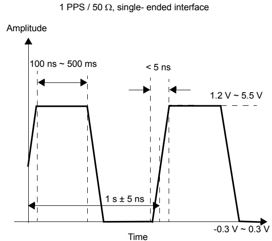
Figure 19 1PPS pulse shape specification in 50 Ω, single ended interfaces. This interface is described in ITU-T G.703 and G.8271.
